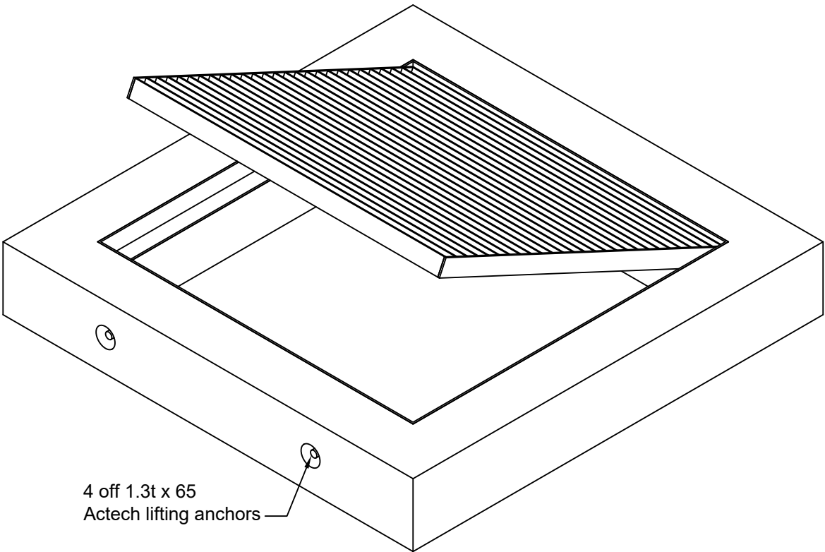
ISOMETRIC VIEW
